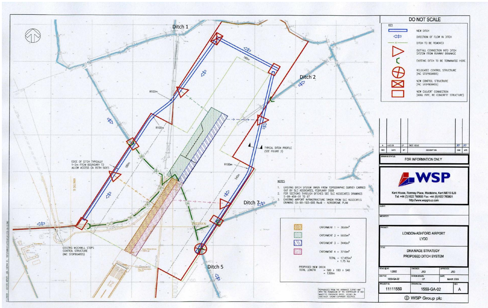
Figure 3 'Loss of SSI application ditches to runway construction'
