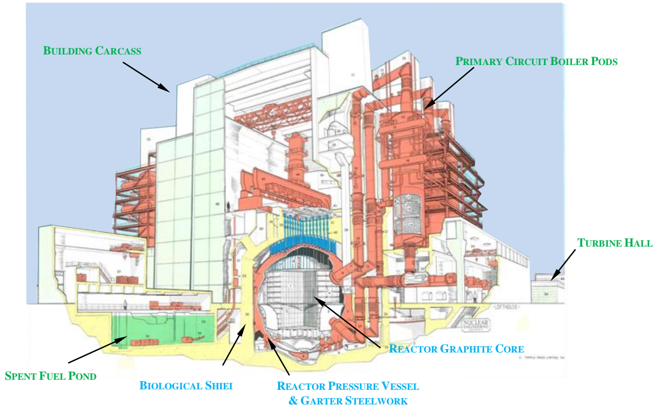
TYPICAL MAGNOX POWER STATION – CUTAWAY SHOWING ONE OF TWO TWIN REACTORS
